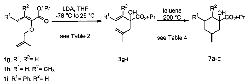
Scheme 5. The sequential ester dienolate [2,3]-Wittig/oxy-Cope rearrangement/type-II ene reaction
