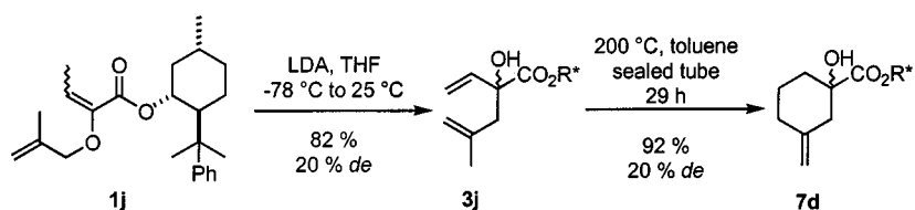
Scheme 7. The attempted auxiliary-controlled domino oxy-Cope rearrangement/type-II ene reaction proved to be inefficient
