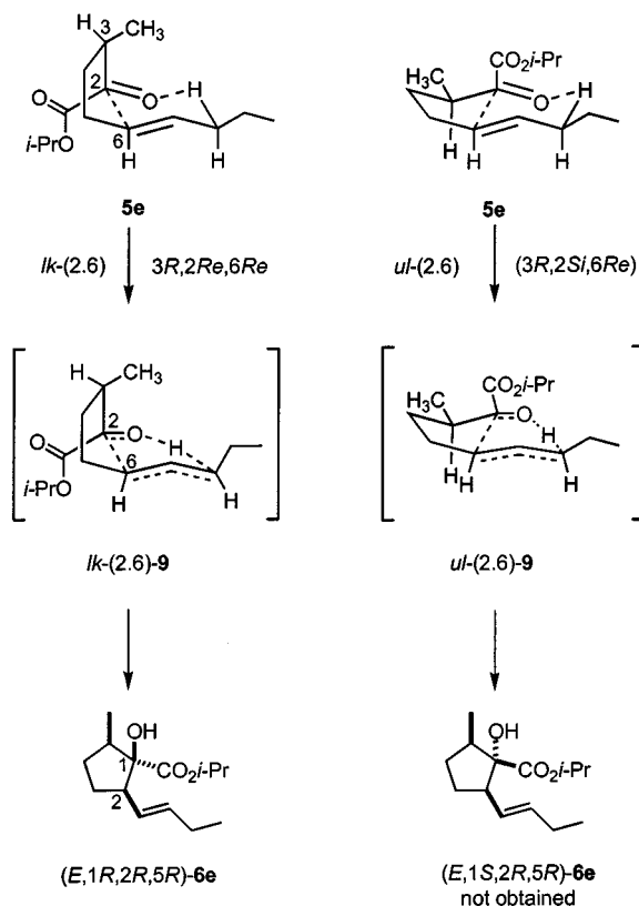
Scheme 4. Proposed transition structures for the type-I ene reaction of the \alpha -oxo ester 5e
