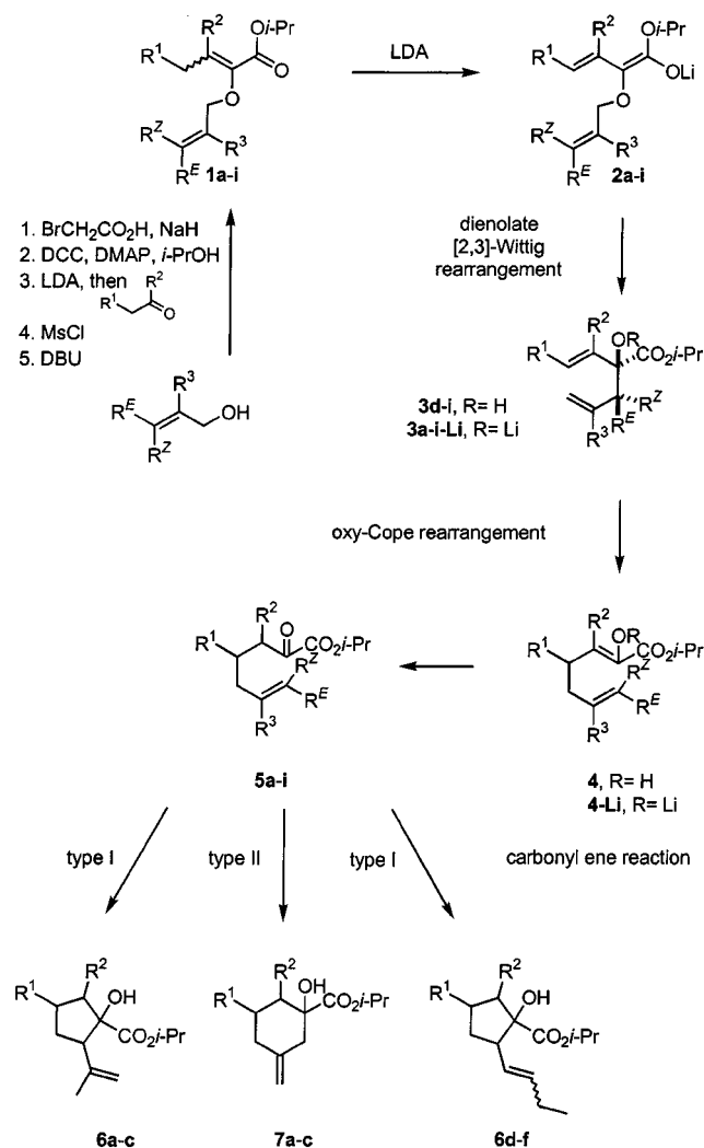
Scheme 1. The sequential dienolate [2,3]-Wittig/oxy-Cope rearrangement/carbonyl ene reaction
