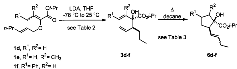
Scheme 3. The sequential ester dienolate [2,3]-Wittig/oxy-Cope rearrangement/type-I ene reaction
