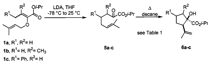
Scheme 2. The sequential ester dienolate [2,3]-Wittig/oxy-Cope rearrangement/type-I ene reaction
