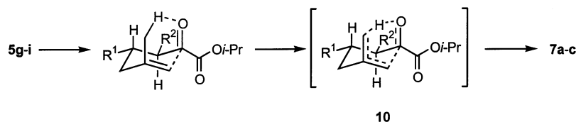
Scheme 6. Proposed transition structures for the type-II ene reaction
